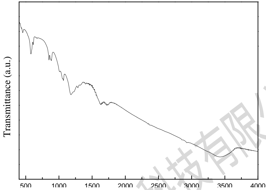
IR of Graphene Oxide
