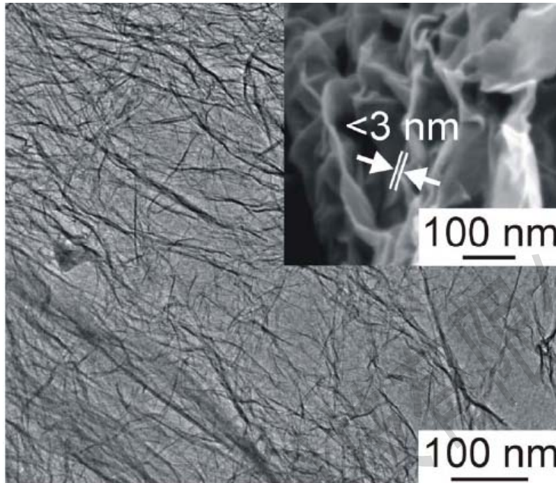
TEM and SEM of Grapheme Oxide
