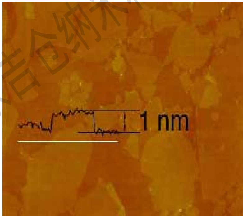
AFM of Graphene Oxide
