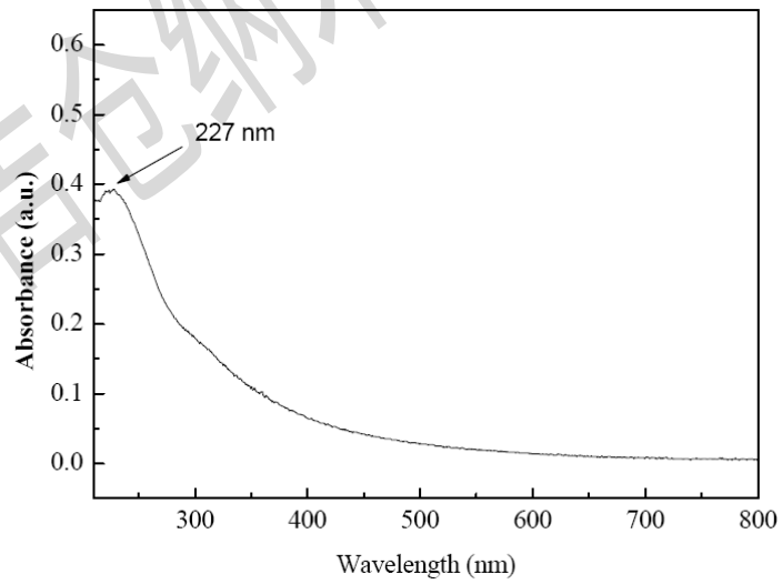
UV of Graphene Oxide
