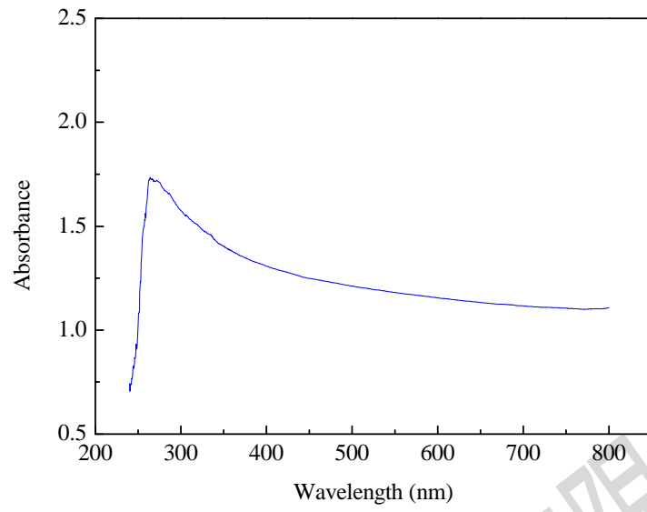
UV of Graphene
